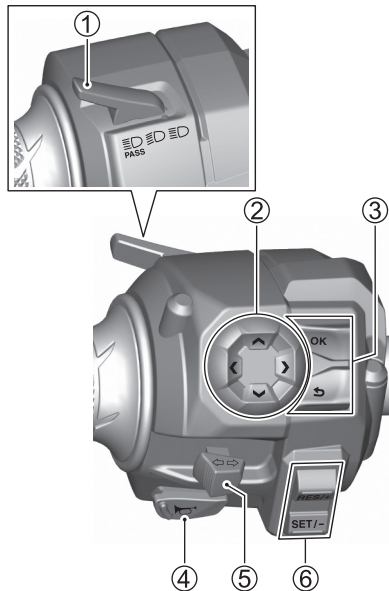
LEFT HANDLEBAR
