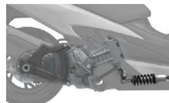
Link-type monoshock rear suspension
