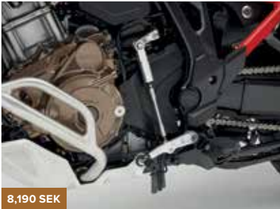
QUICK SHIFTER 08U70-MKK-D01 Made of stainless steel and featuring By measuring the intensity of the shifting input, the quick shifter enables the rider to change gears without operating the clutch lever or shutting the throttle. The system works for upshifting and downshifting, maximizing the riding experience. (For MT version only).
